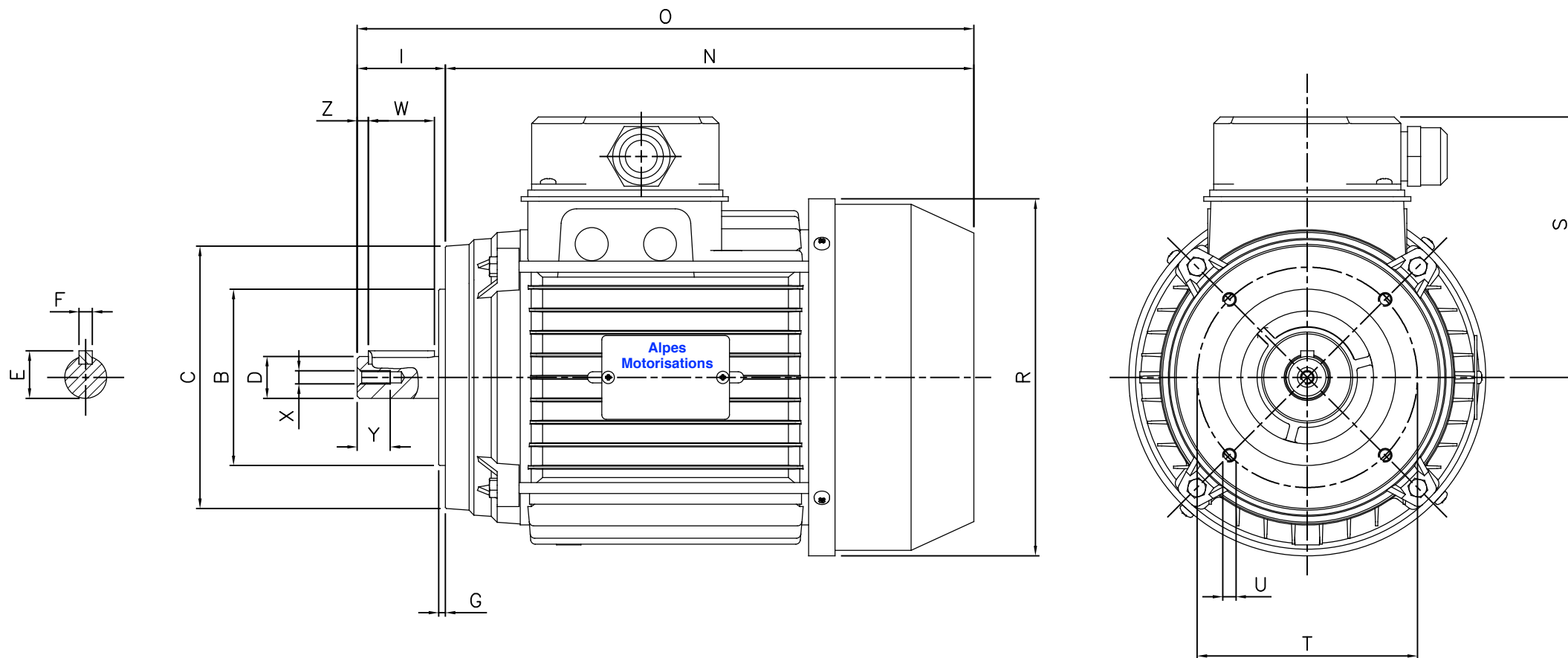
FORMA B14 – DIMENSIONI / FRAME SIZE B14 FORM
